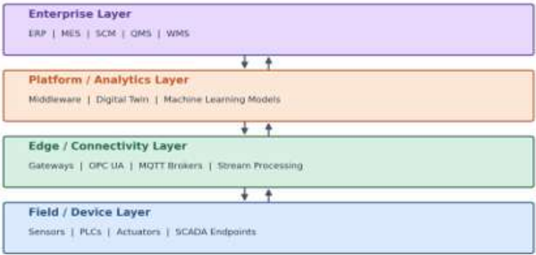
Figure 1. Layered Architecture for Iot-Enabled Enterprise Integration, Showing Bidirectional Data Exchange between Field Devices and Enterprise Applications
